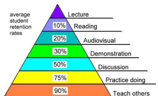
Learning Pyramid
